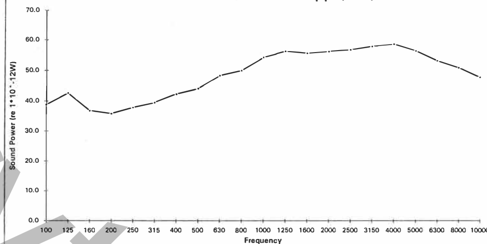
Noise Level From bare 100mm PVC pipe (No 1)
